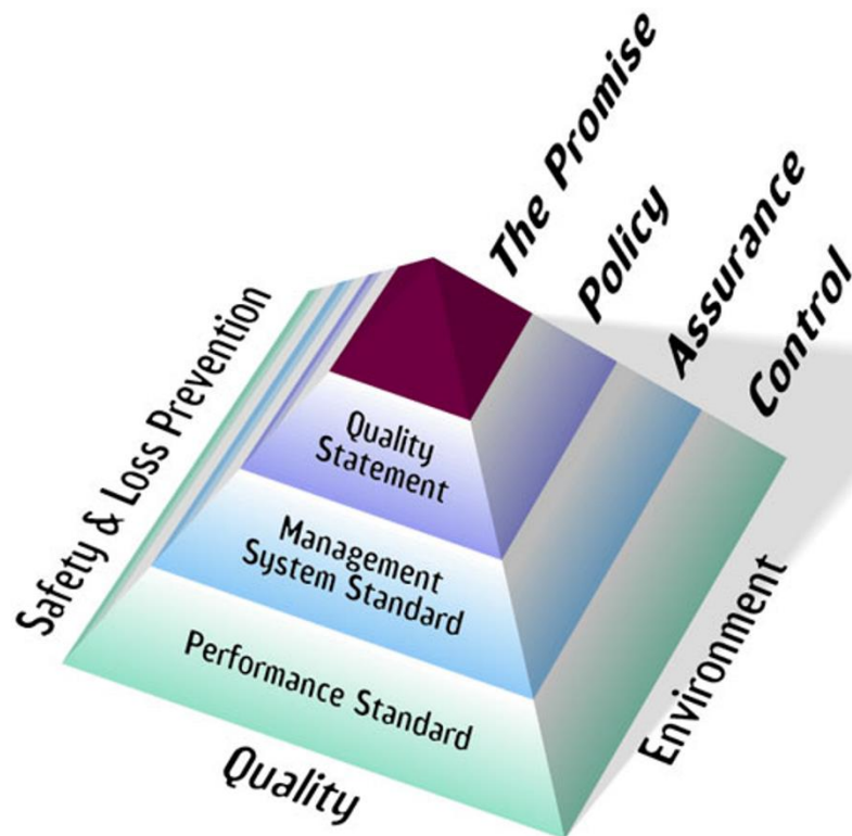
Process pyramid
